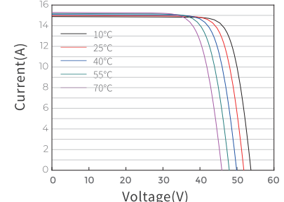
Current-Voltage Curve JAM72D42-620/LB
