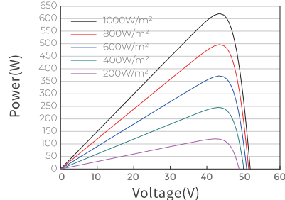
Power-Voltage Curve JAM72D42-620/LB
